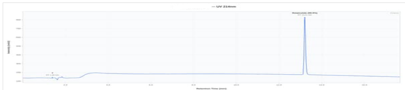
Opti-(R) 20mg - OS-2026-7564: UV Chromatogram
