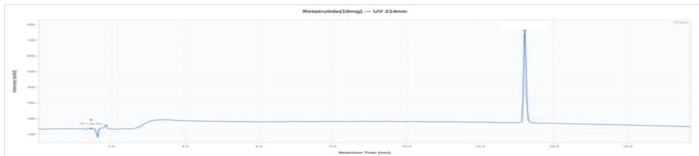
Opti-(R) 10mg - OS-2026-7564: UV Chromatogram
