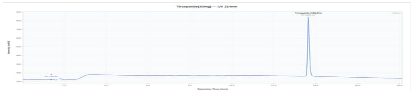
Opti-(T) 30mg - OS-2026-7253: UV Chromatogram
