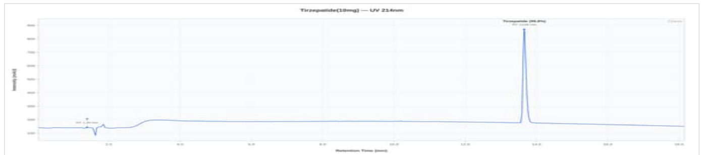
Opti-(T) 10mg - OS-2026-7253: UV Chromatogram
