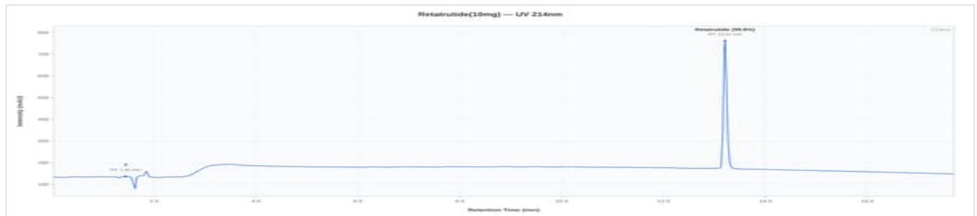
Opti-(R) 10mg - OS-2026-7564: UV Chromatogram
